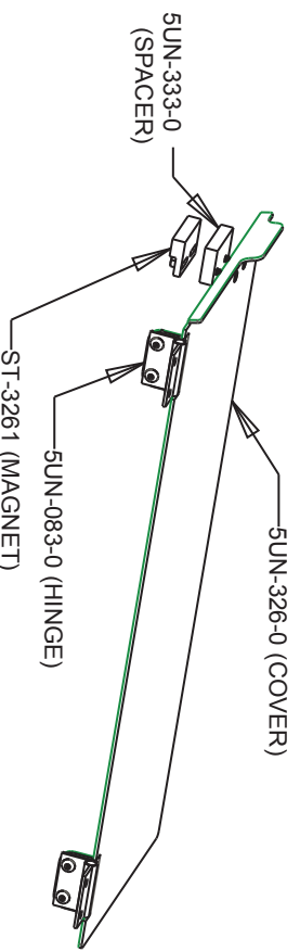
ITEM 33 - TOP COVER & HINGE ASSY 5UN-326-1
