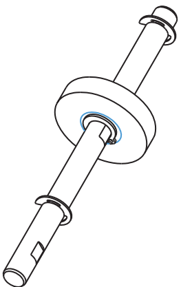
ITEM 7 - FEED WHEEL SHAFT ASSY 5UN-025-1
