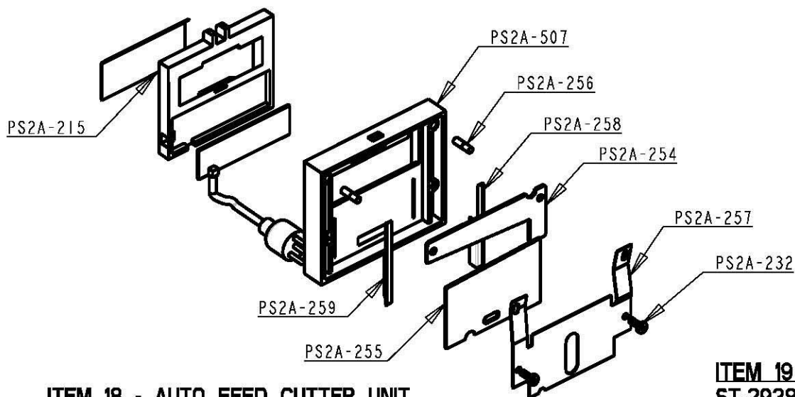
ITEM 18 - AUTO FEED CUTTER UNIT PS2A-550 - ONLY SOLD AS COMPLETE ASSEMBLY
